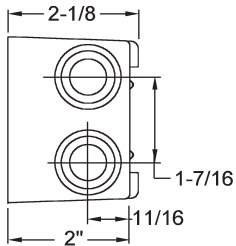
END VIEW TWO OUTLET
